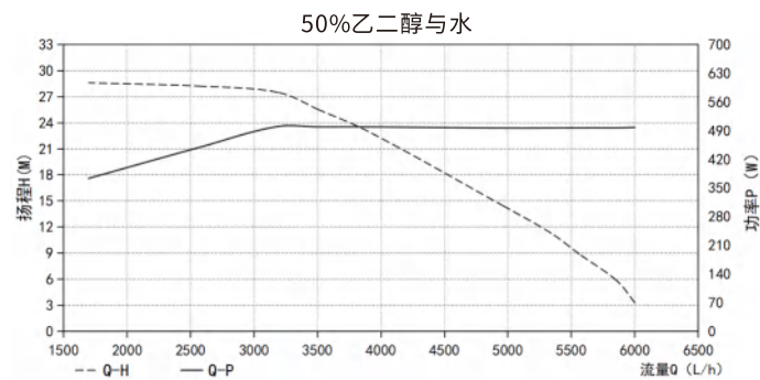
流量扬程图 Pump Performance Curve
