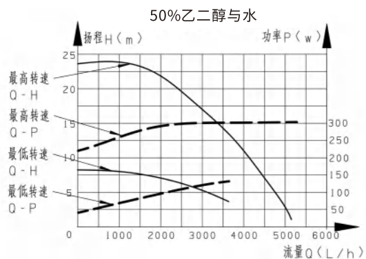
流量扬程图 Pump Performance Curve
