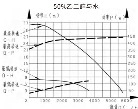
流量扬程图 Pump Performance Curve
