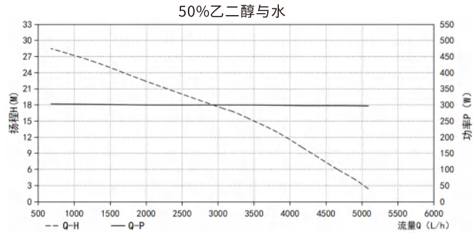
流量扬程图 Pump Performance Curve
