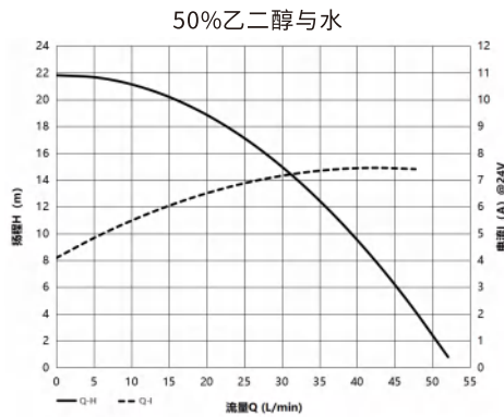
流量扬程图 Pump Performance Curve
