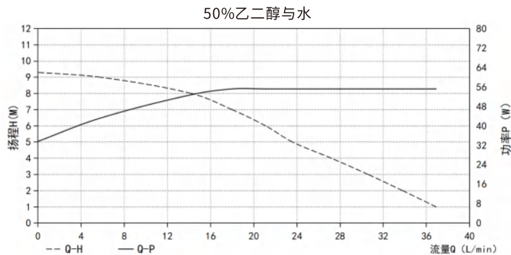
流量扬程图 Pump Performance Curve
